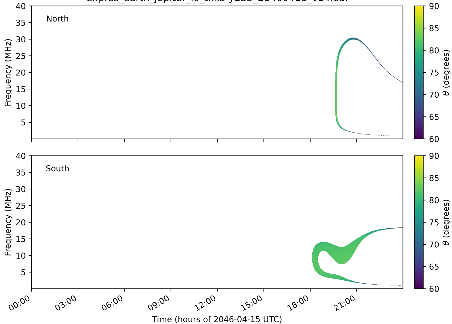
expres_earth_jupiter_io_txka-y235_20460415_v14.cdf
