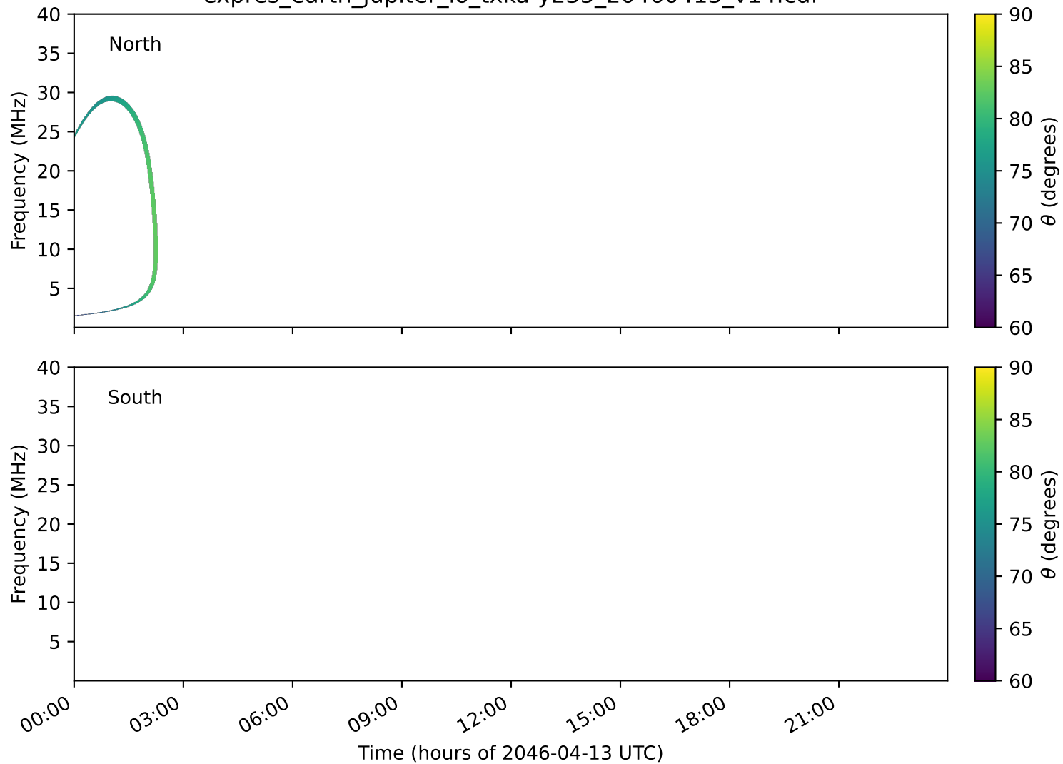
expres_earth_jupiter_io_txka-y235_20460413_v14.cdf
