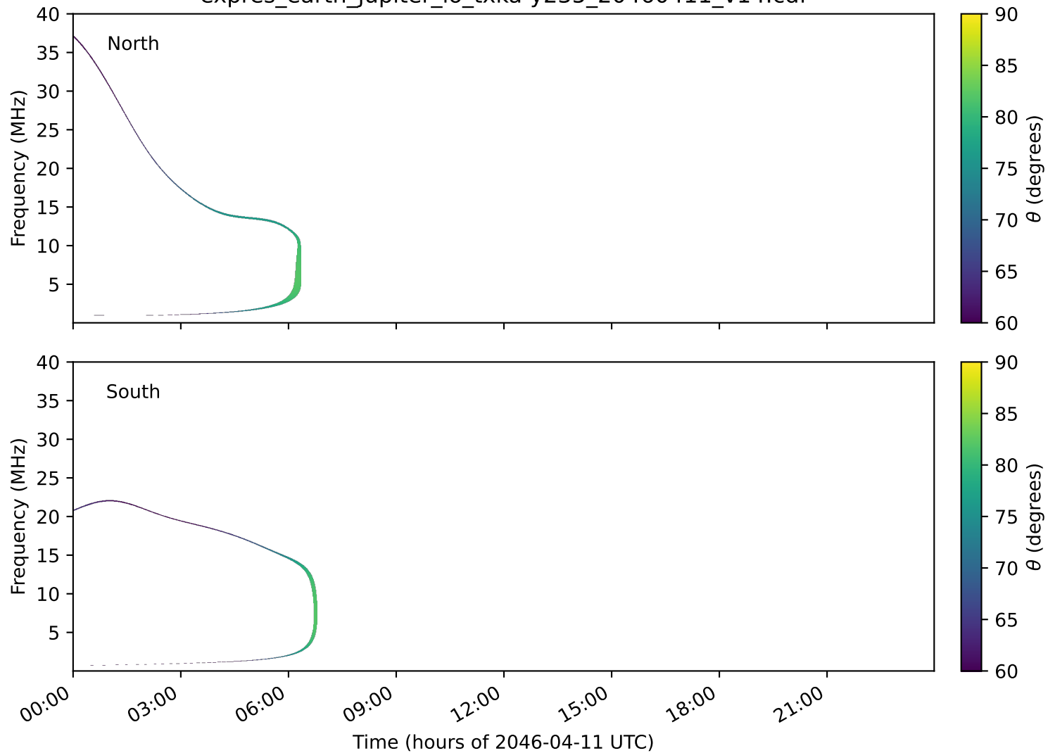
expres_earth_jupiter_io_txka-y235_20460411_v14.cdf
