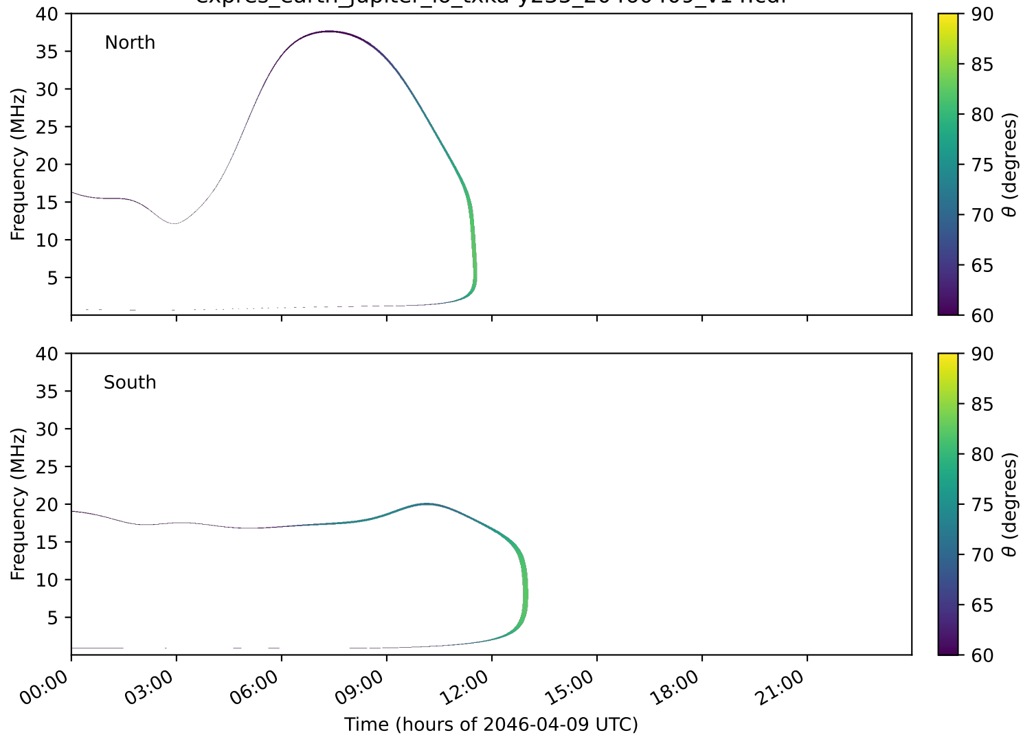
expres_earth_jupiter_io_txka-y235_20460409_v14.cdf
