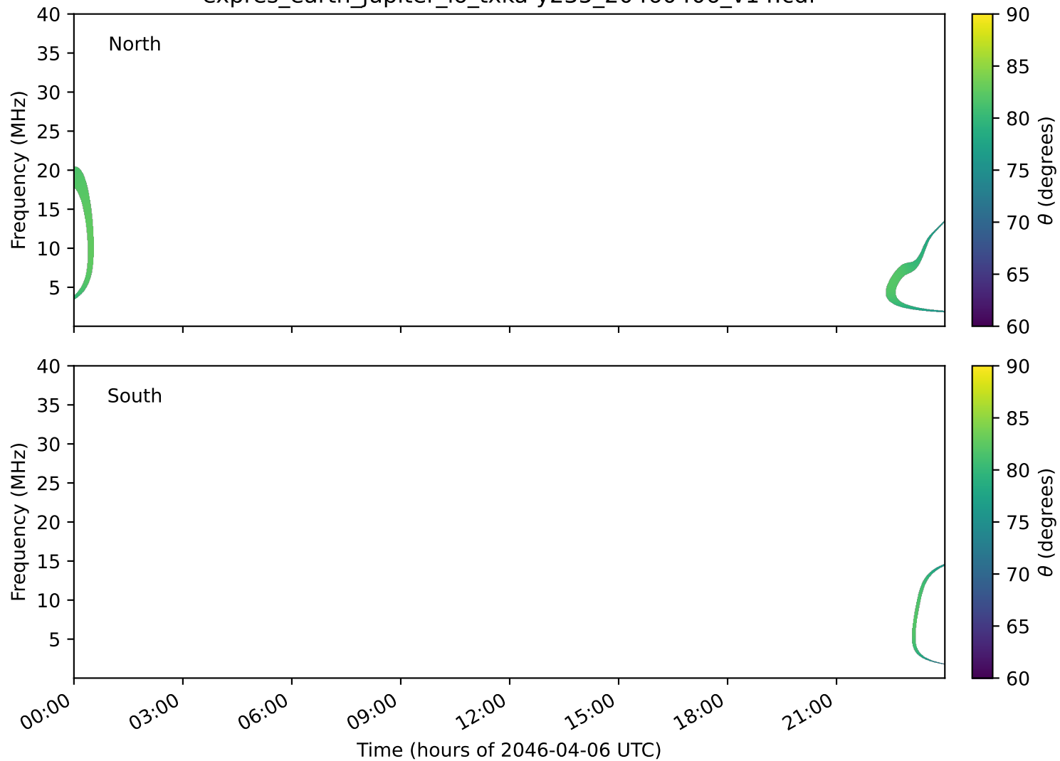
expres_earth_jupiter_io_txka-y235_20460406_v14.cdf
