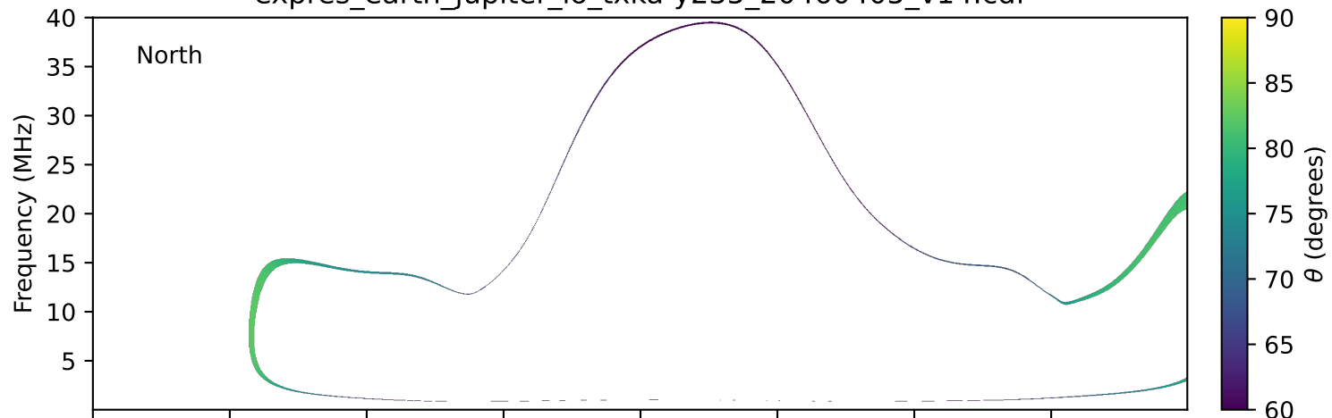
expres_earth_jupiter_io_txka-y235_20460405_v14.cdf
