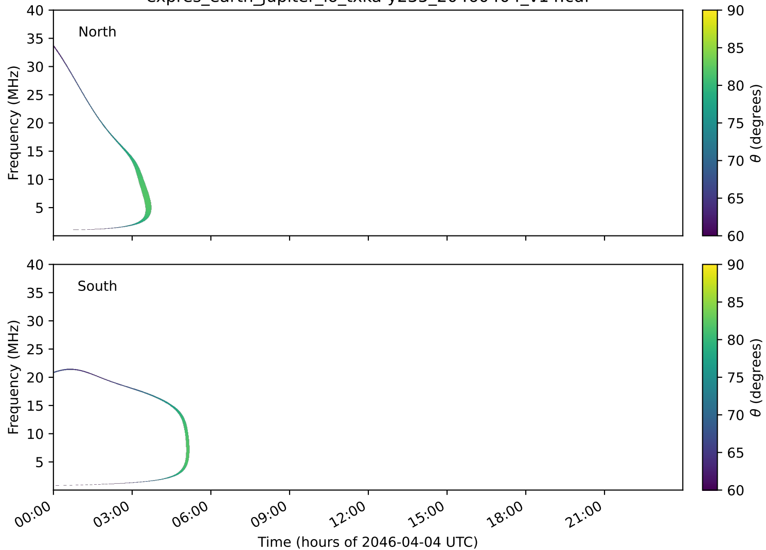
expres_earth_jupiter_io_txka-y235_20460404_v14.cdf
