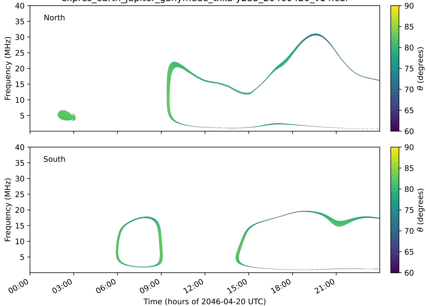
expres_earth_jupiter_ganymede_txka-y235_20460420_v14.cdf
