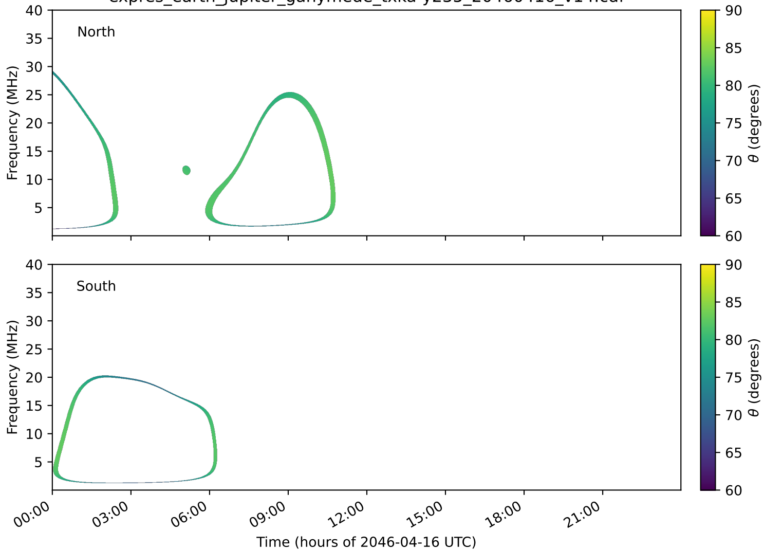
expres_earth_jupiter_ganymede_txka-y235_20460416_v14.cdf
