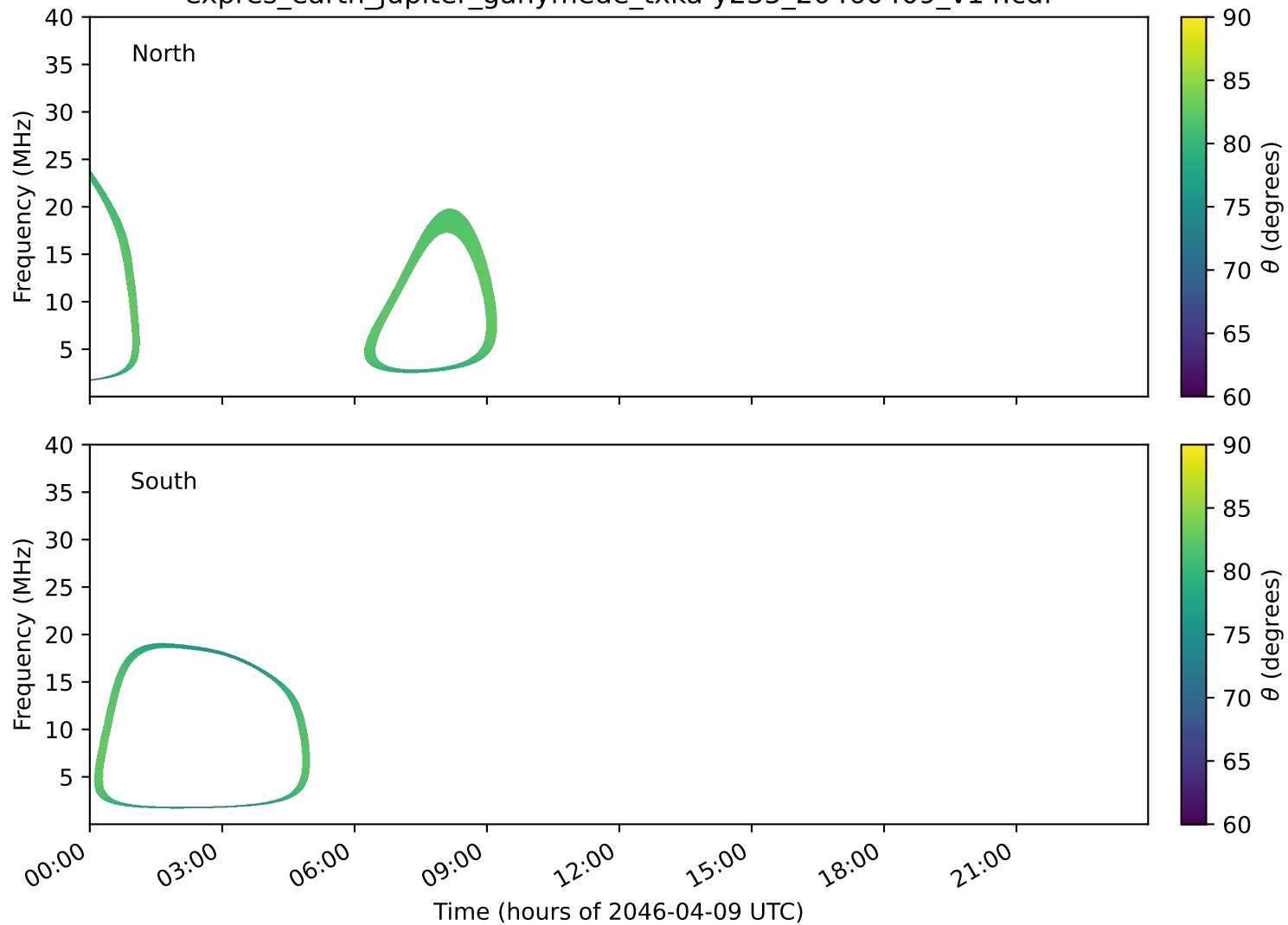
expres_earth_jupiter_ganymede_txka-y235_20460409_v14.cdf
