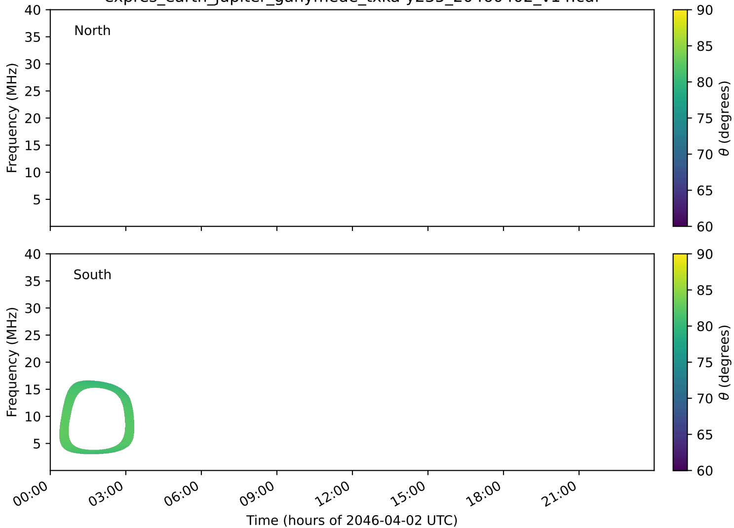
expres_earth_jupiter_ganymede_txka-y235_20460402_v14.cdf
