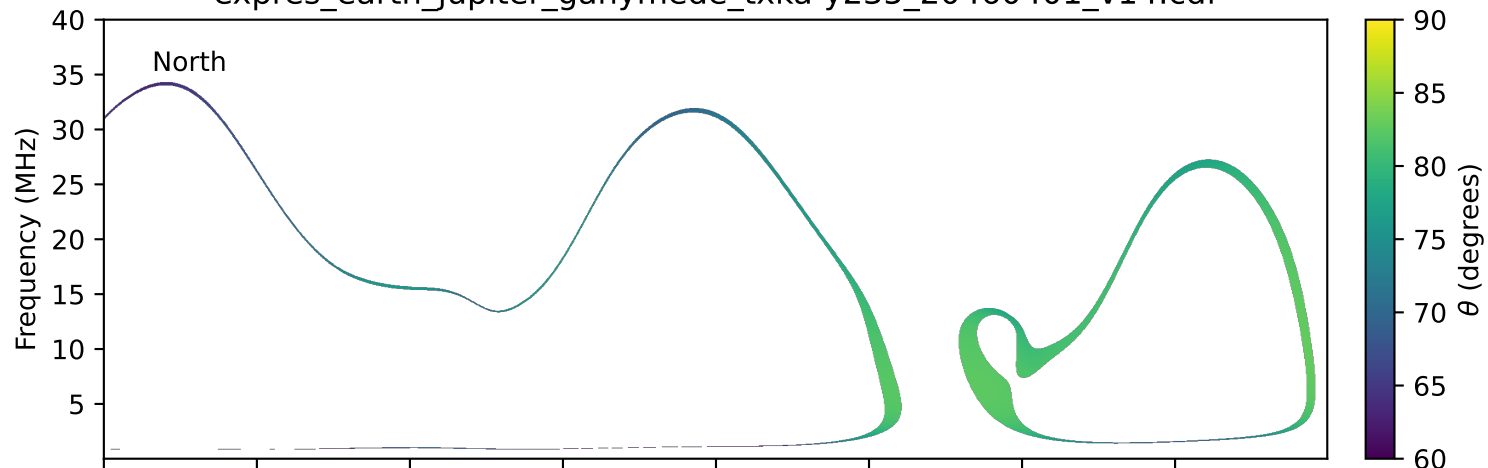
expres_earth_jupiter_ganymede_txka-y235_20460401_v14.cdf
