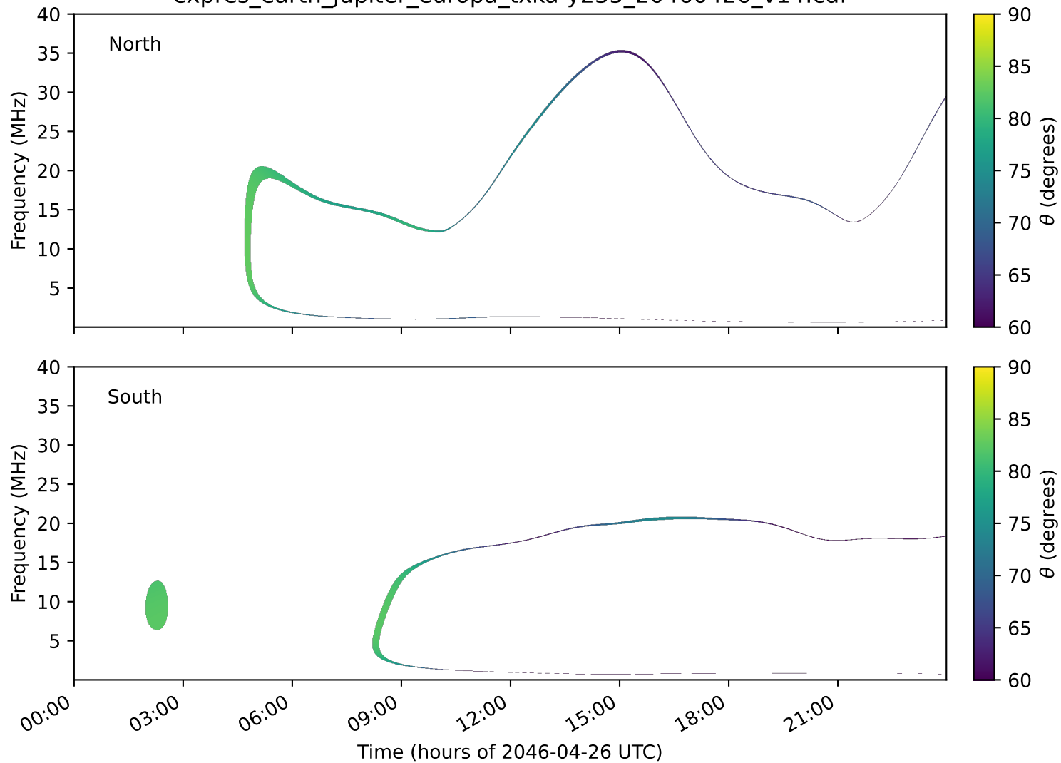
expres_earth_jupiter_europa_txka-y235_20460426_v14.cdf
