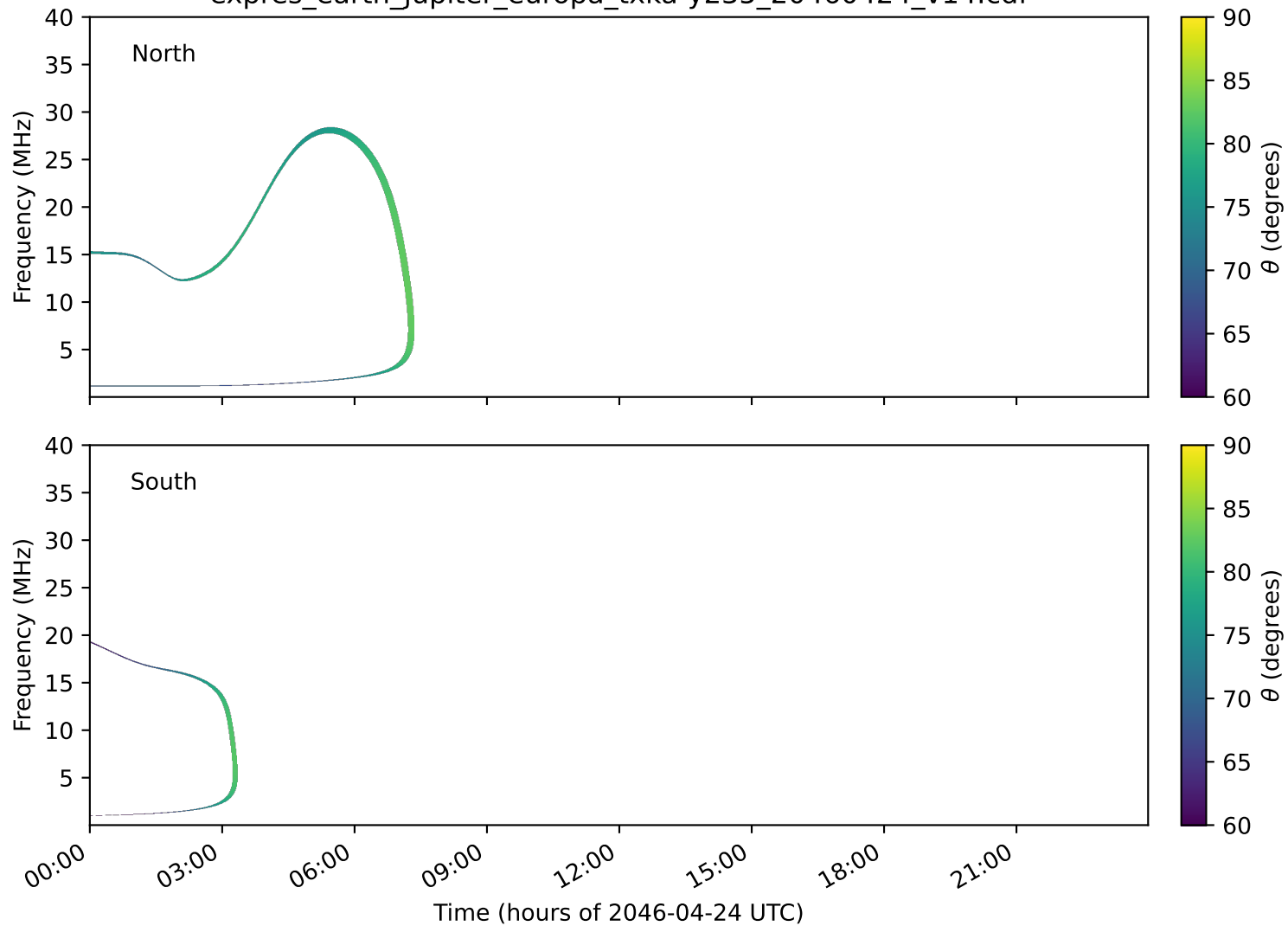
expres_earth_jupiter_europa_txka-y235_20460424_v14.cdf
