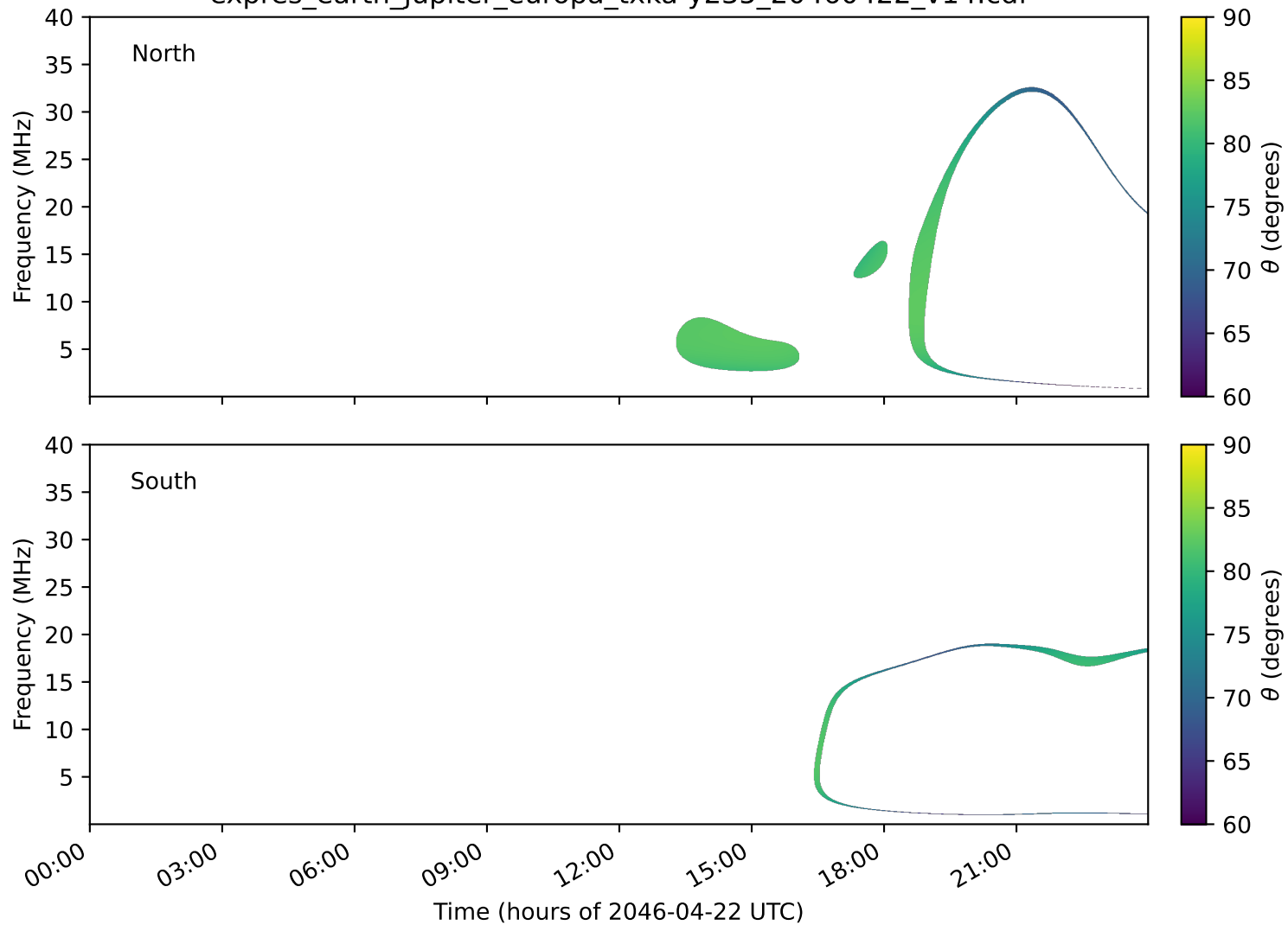
expres_earth_jupiter_europa_txka-y235_20460422_v14.cdf
