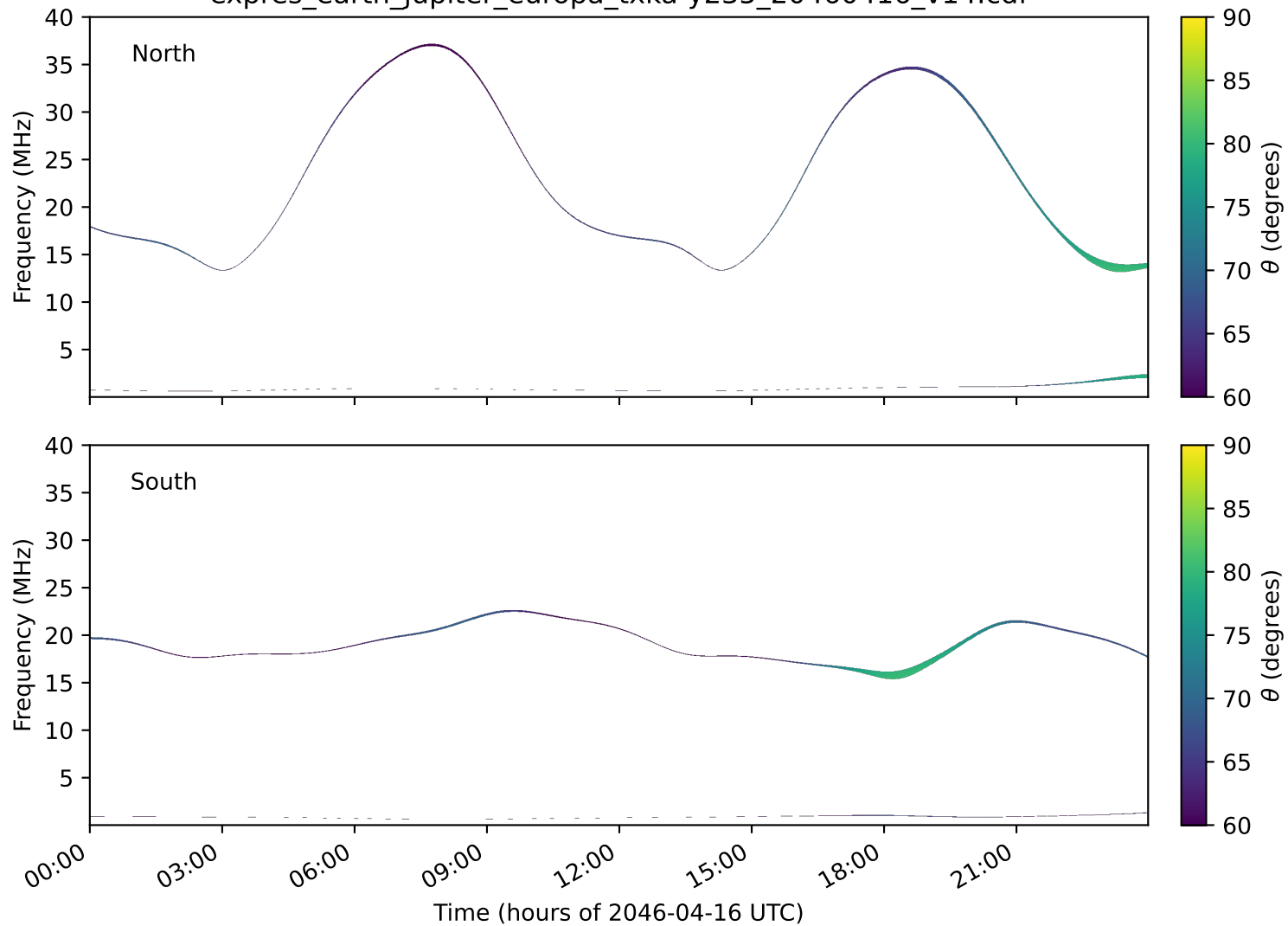
expres_earth_jupiter_europa_txka-y235_20460416_v14.cdf
