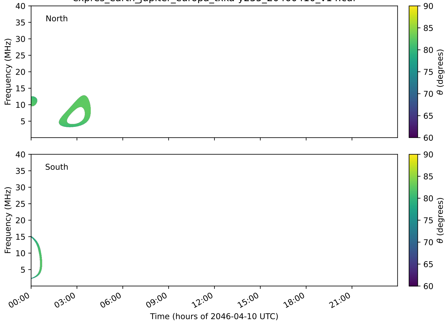
expres_earth_jupiter_europa_txka-y235_20460410_v14.cdf
