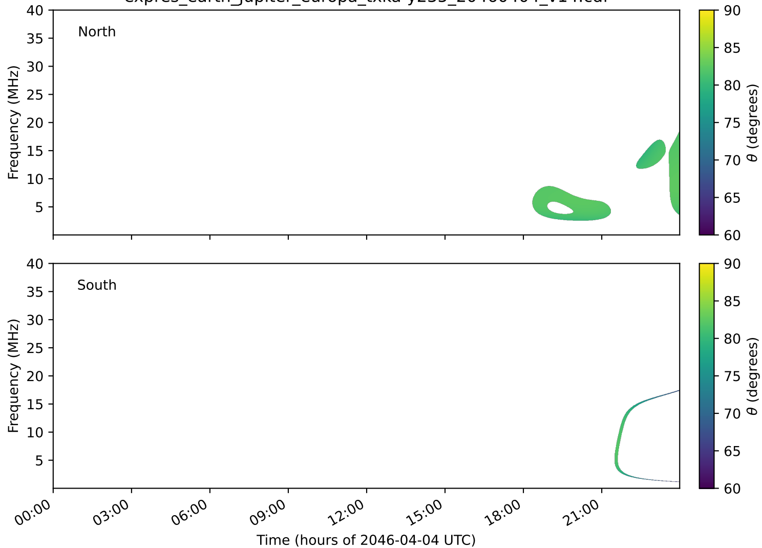
expres_earth_jupiter_europa_txka-y235_20460404_v14.cdf
