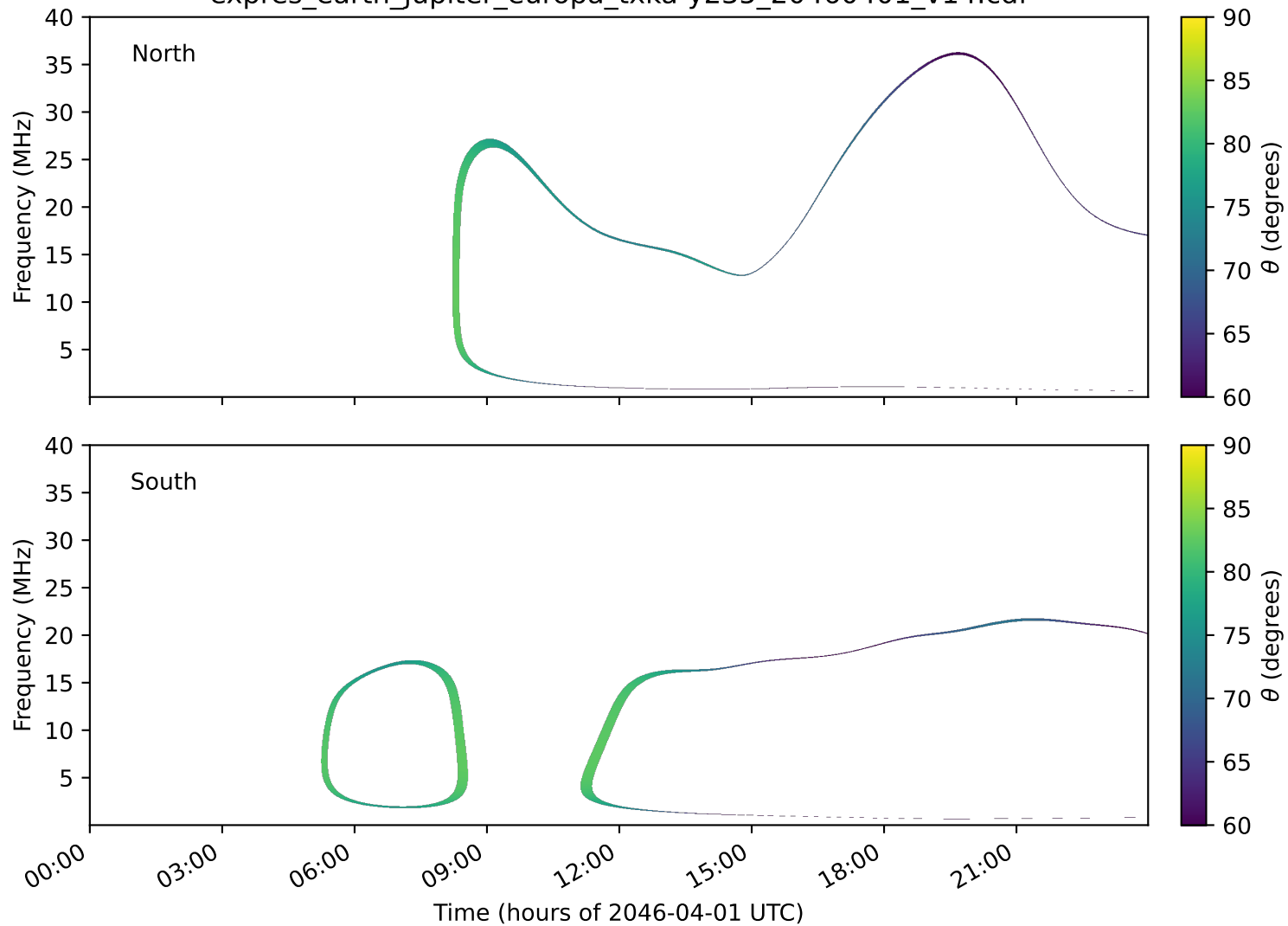
expres_earth_jupiter_europa_txka-y235_20460401_v14.cdf
