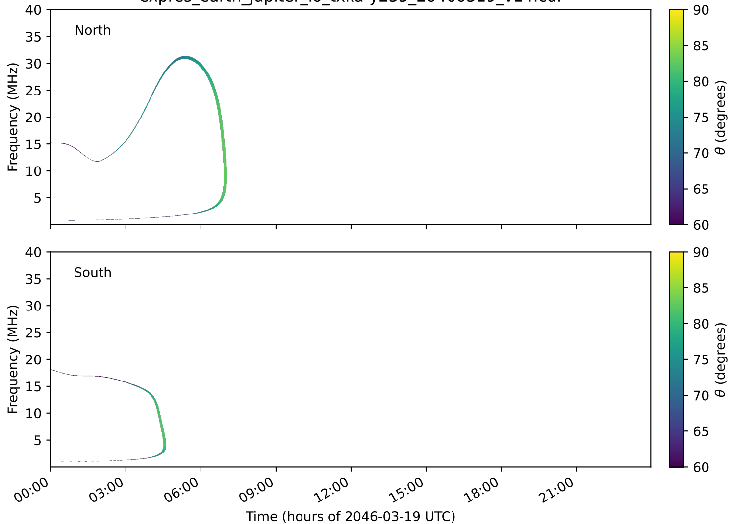
expres_earth_jupiter_io_txka-y235_20460319_v14.cdf
