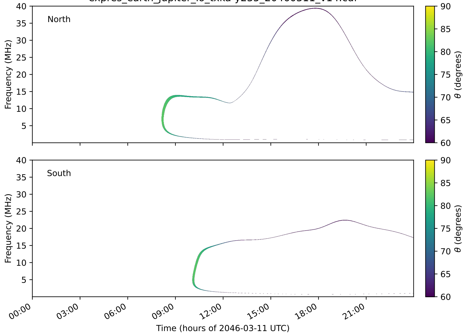
expres_earth_jupiter_io_txka-y235_20460311_v14.cdf
