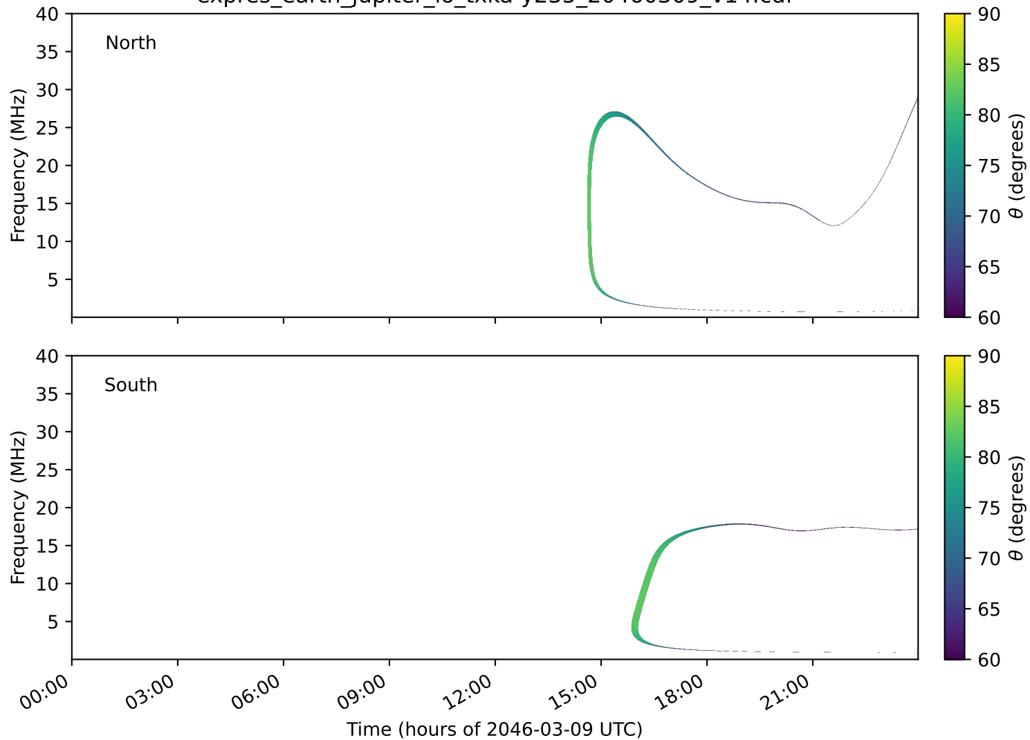
expres_earth_jupiter_io_txka-y235_20460309_v14.cdf
