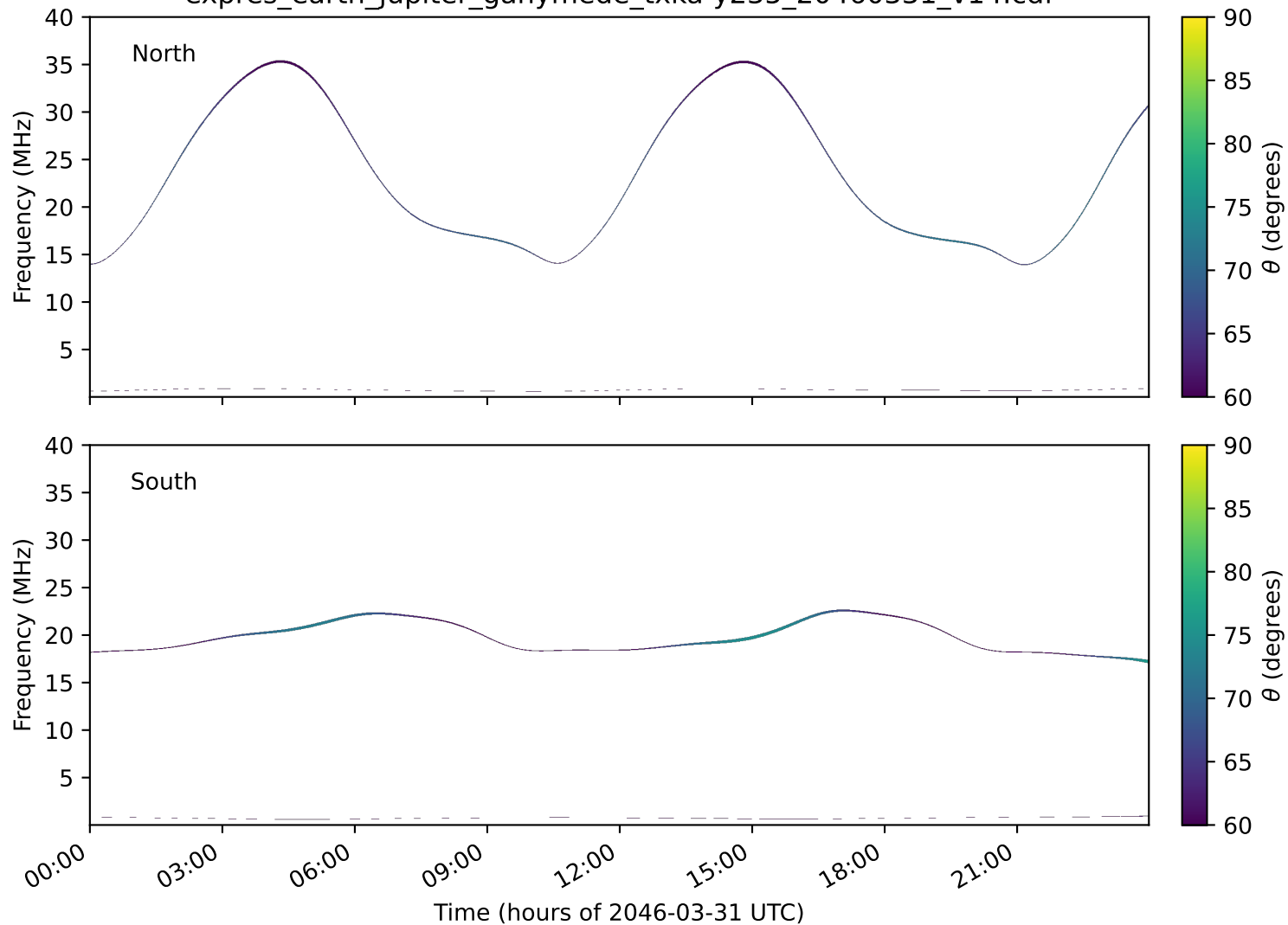
expres_earth_jupiter_ganymede_txka-y235_20460331_v14.cdf
