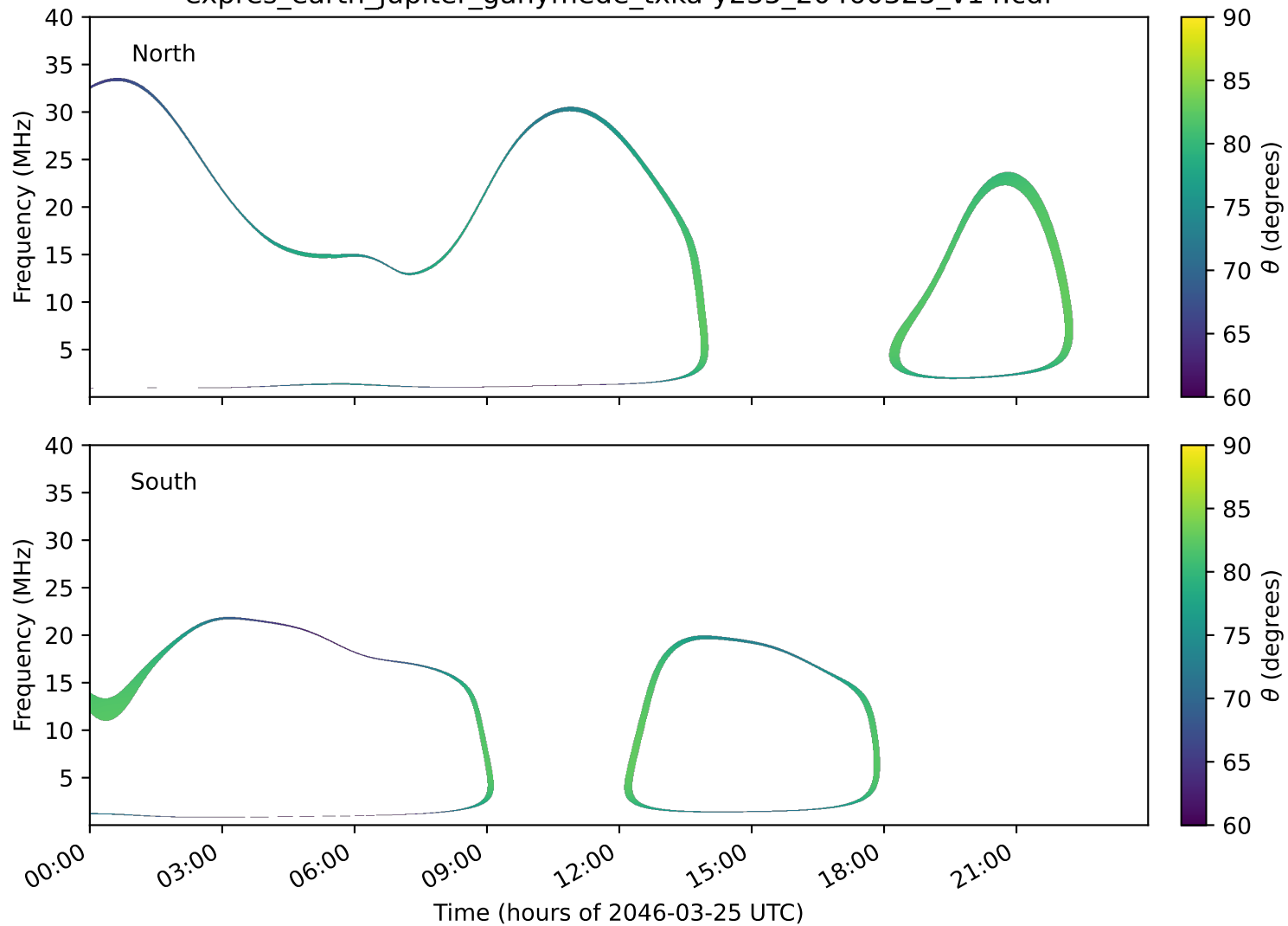
expres_earth_jupiter_ganymede_txka-y235_20460325_v14.cdf
