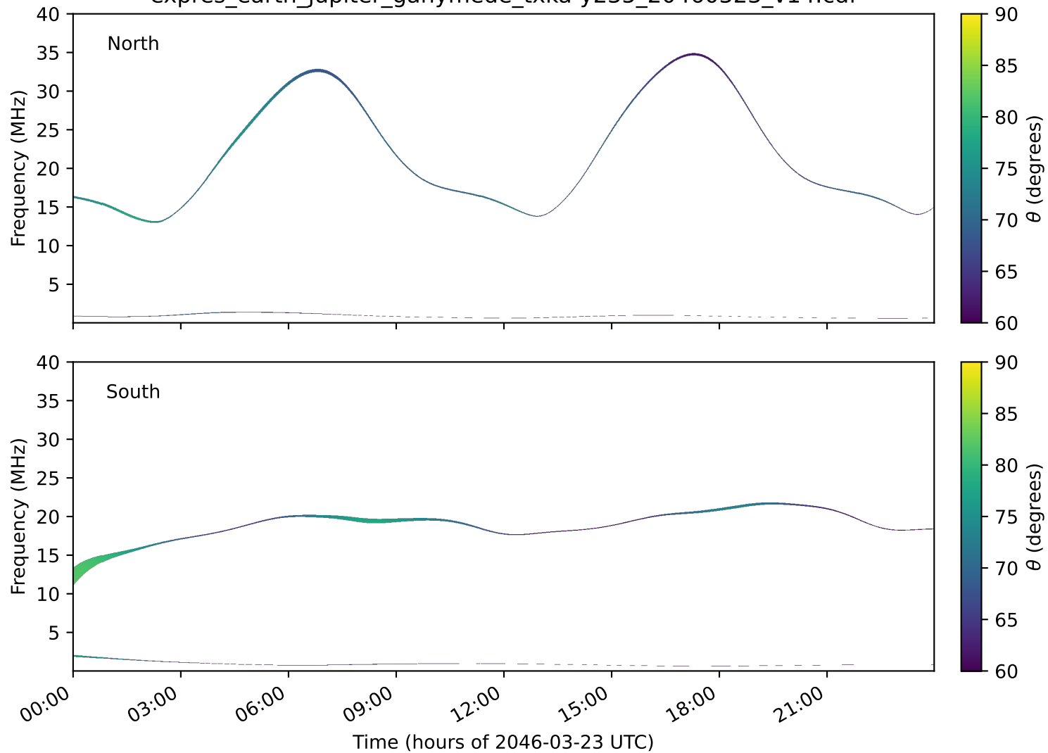
expres_earth_jupiter_ganymede_txka-y235_20460323_v14.cdf
