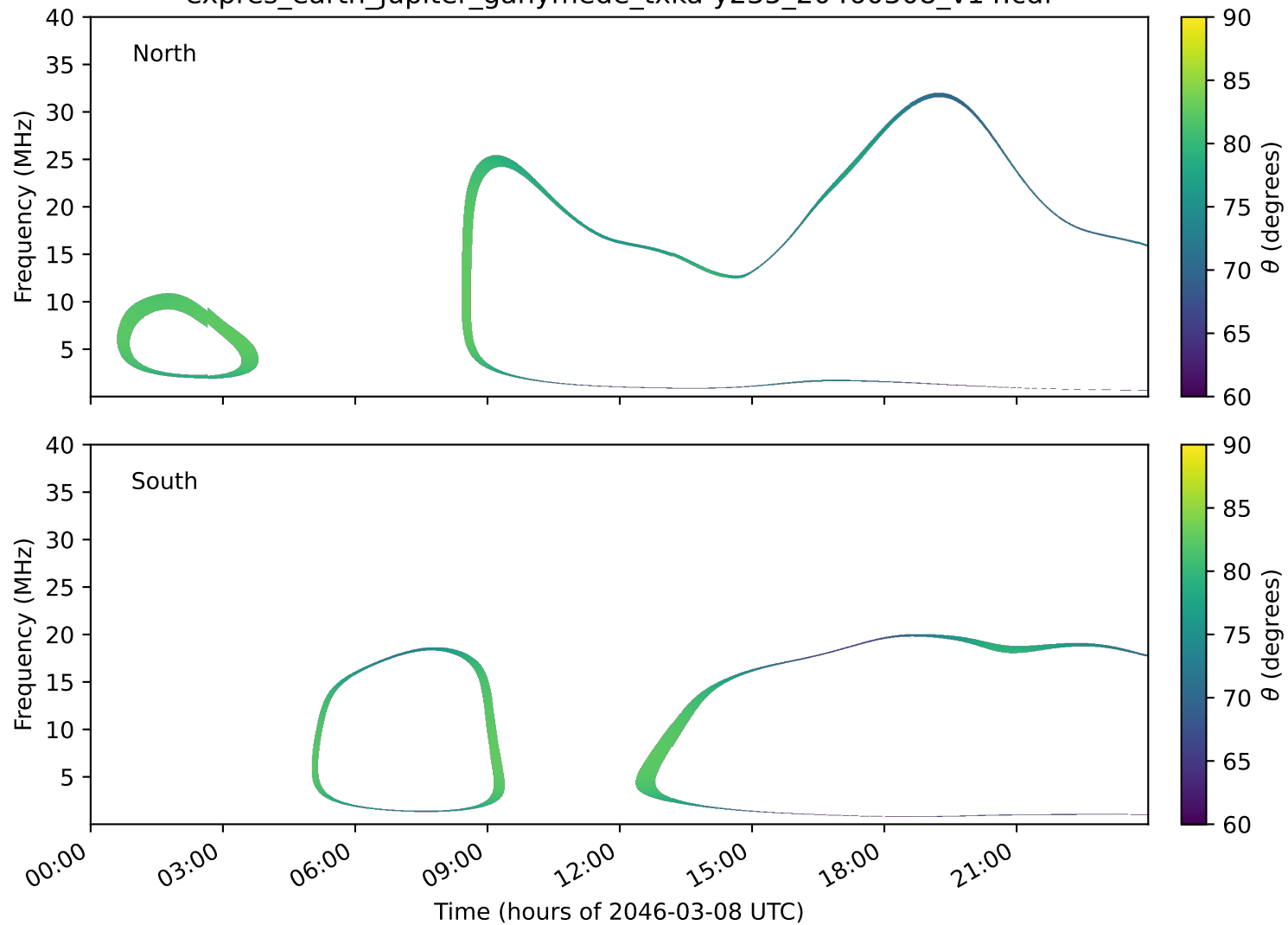
expres_earth_jupiter_ganymede_txka-y235_20460308_v14.cdf
