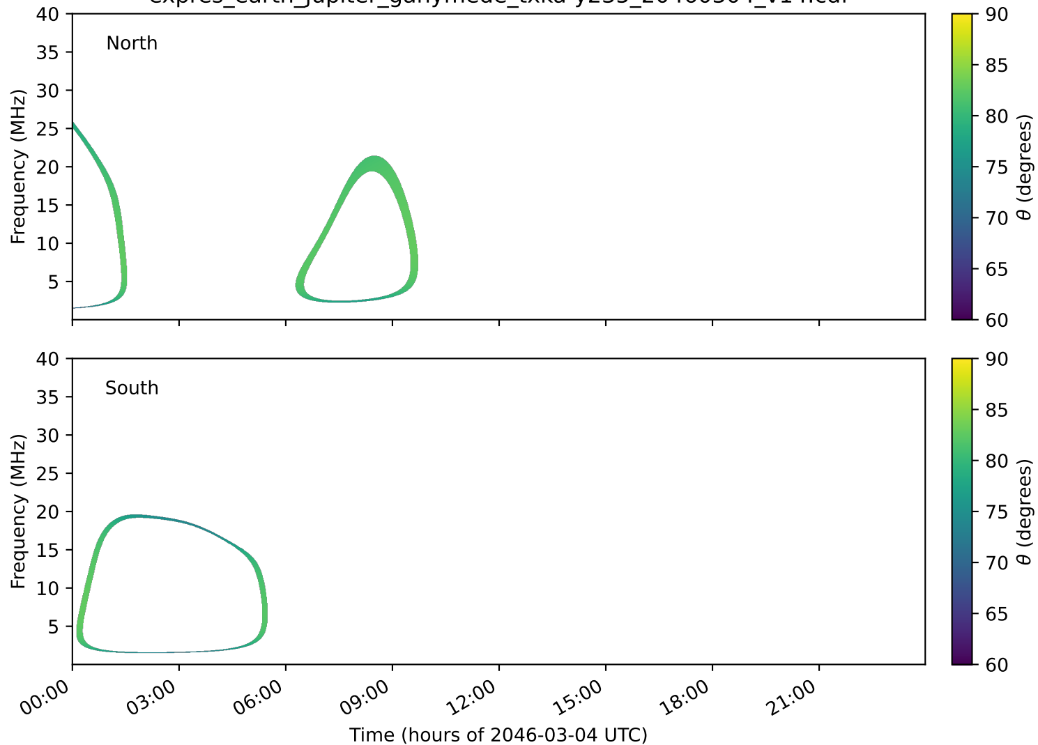
expres_earth_jupiter_ganymede_txka-y235_20460304_v14.cdf
