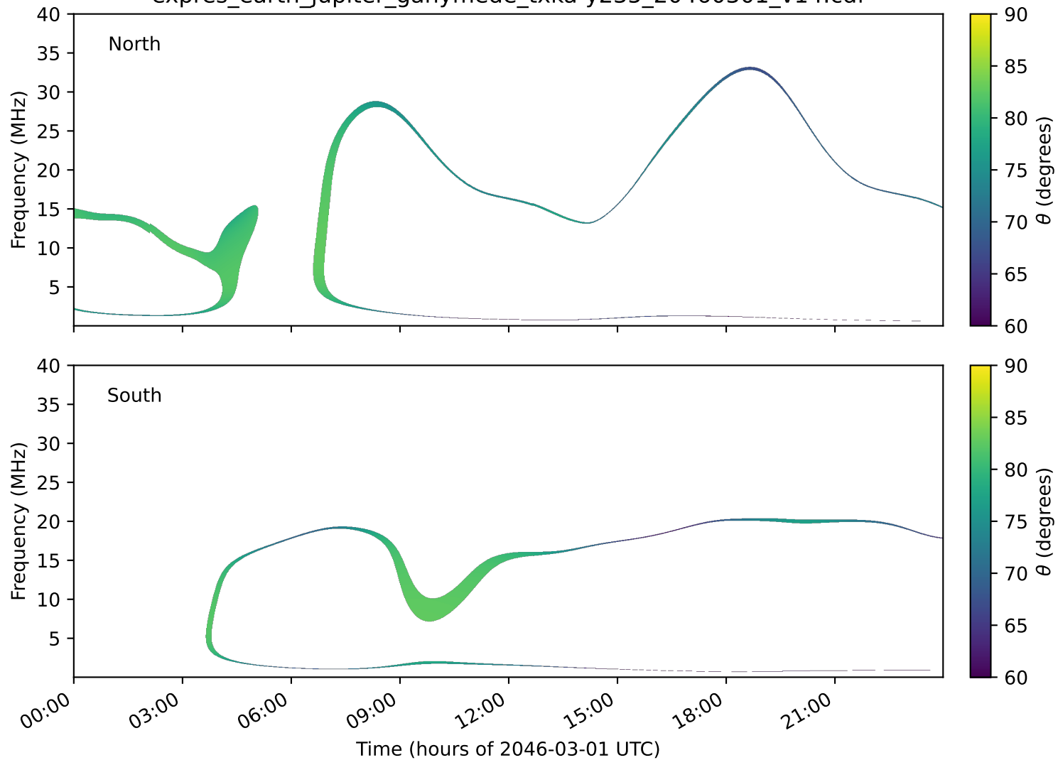
expres_earth_jupiter_ganymede_txka-y235_20460301_v14.cdf
