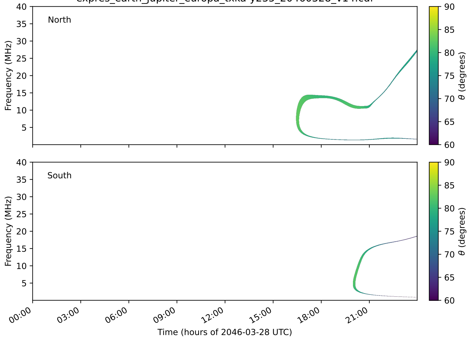
expres_earth_jupiter_europa_txka-y235_20460328_v14.cdf
