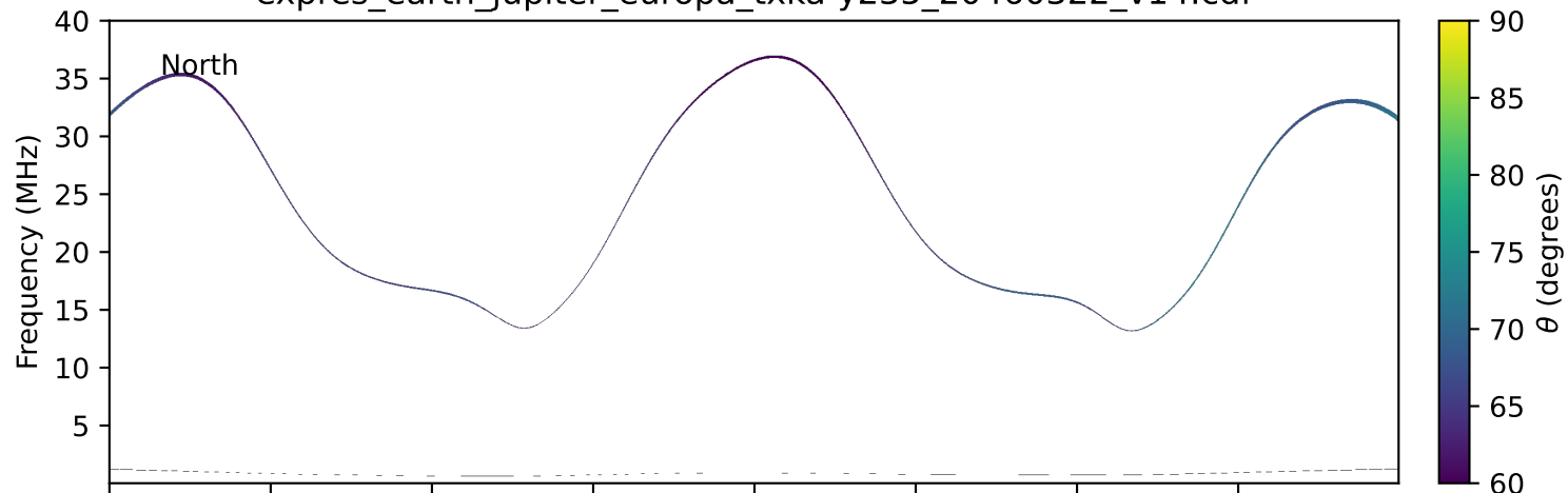
expres_earth_jupiter_europa_txka-y235_20460322_v14.cdf
