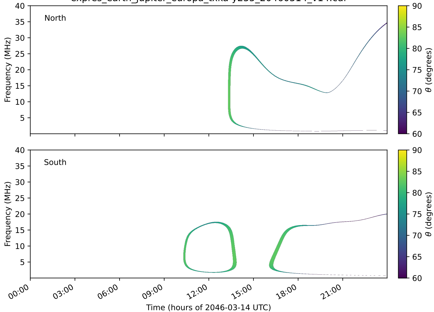
expres_earth_jupiter_europa_txka-y235_20460314_v14.cdf
