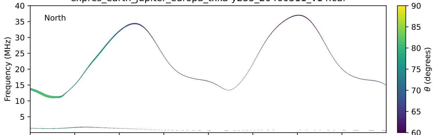
expres_earth_jupiter_europa_txka-y235_20460311_v14.cdf
