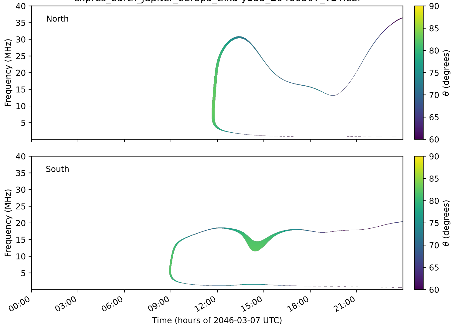
expres_earth_jupiter_europa_txka-y235_20460307_v14.cdf
