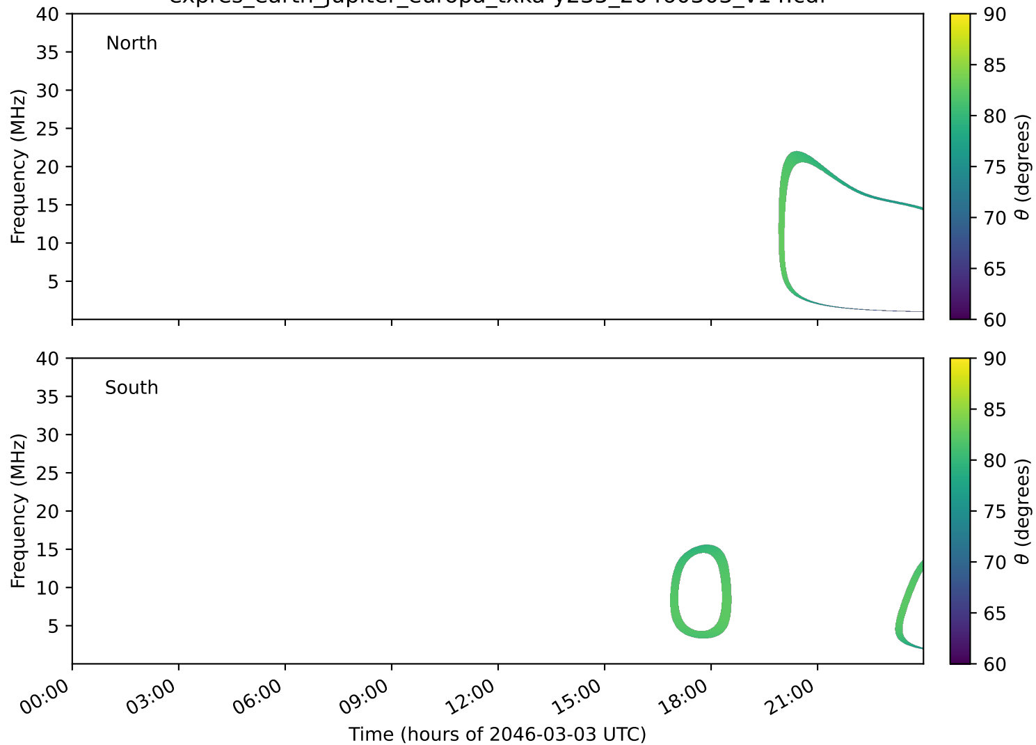
expres_earth_jupiter_europa_txka-y235_20460303_v14.cdf
