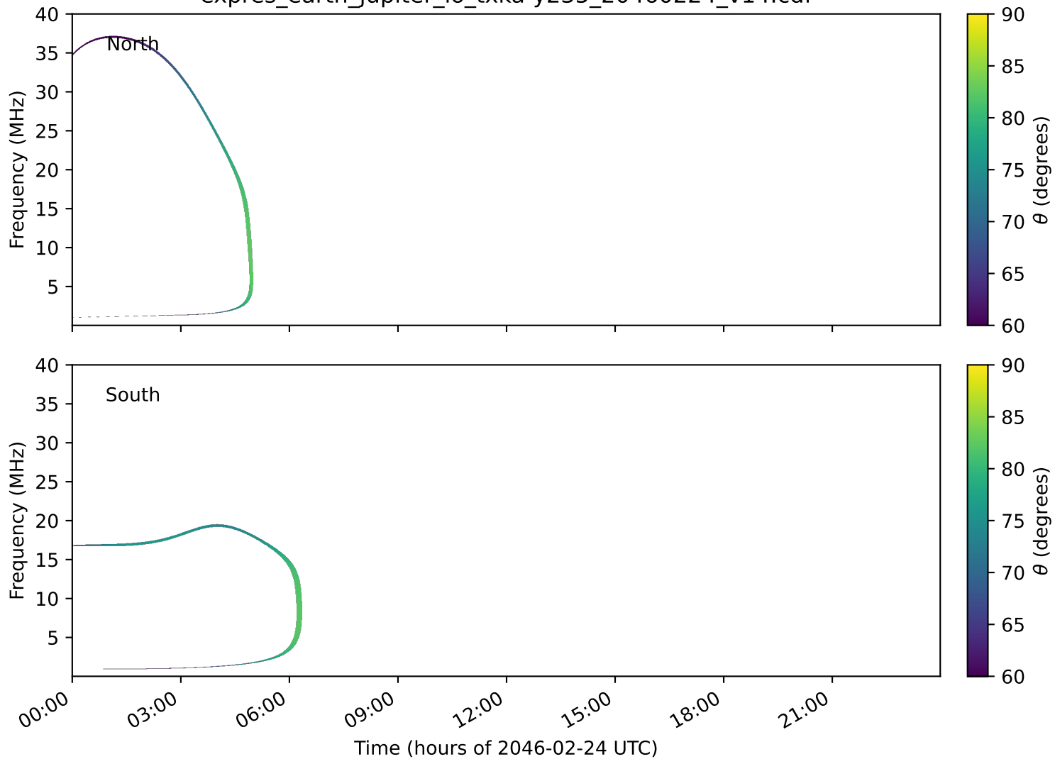
expres_earth_jupiter_io_txka-y235_20460224_v14.cdf
