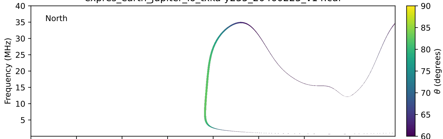
expres_earth_jupiter_io_txka-y235_20460223_v14.cdf
