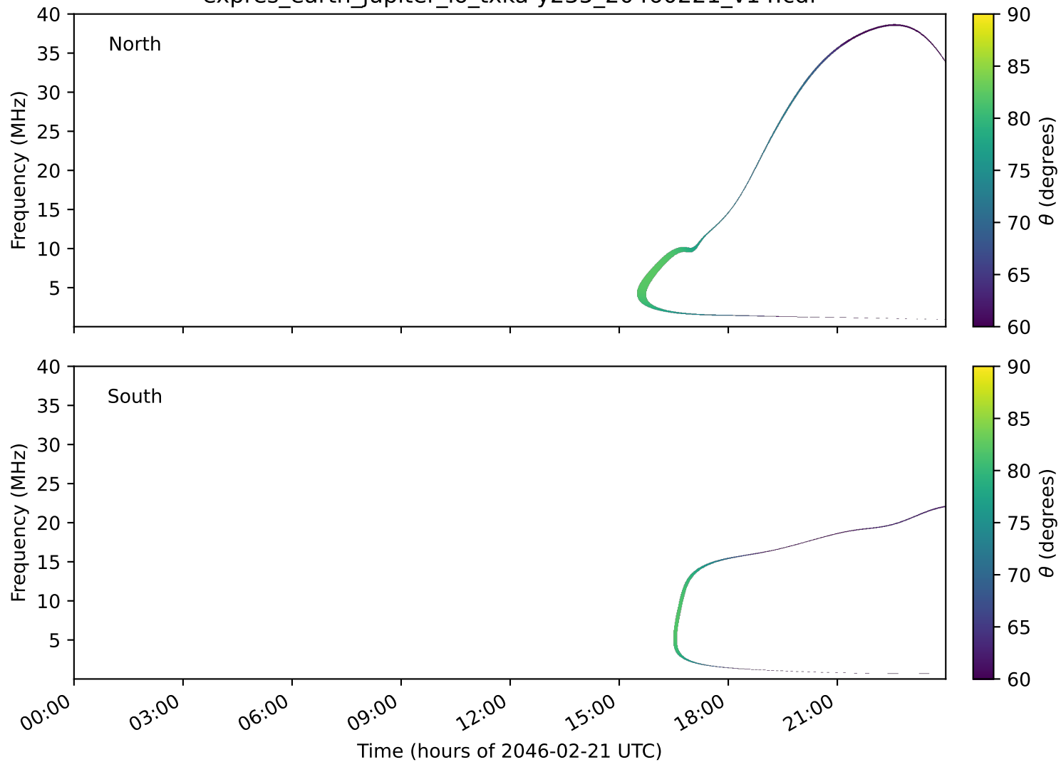
expres_earth_jupiter_io_txka-y235_20460221_v14.cdf
