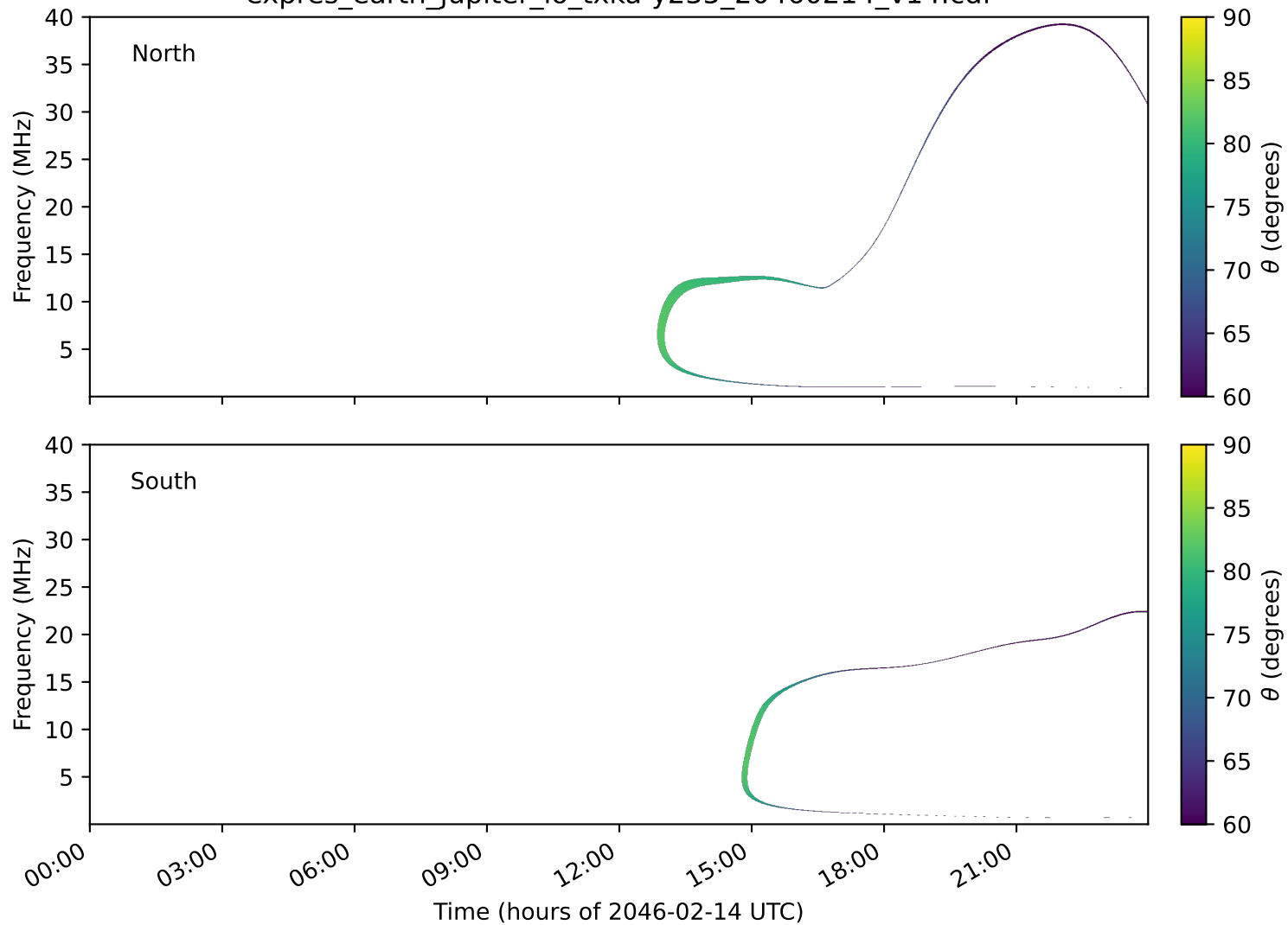
expres_earth_jupiter_io_txka-y235_20460214_v14.cdf
