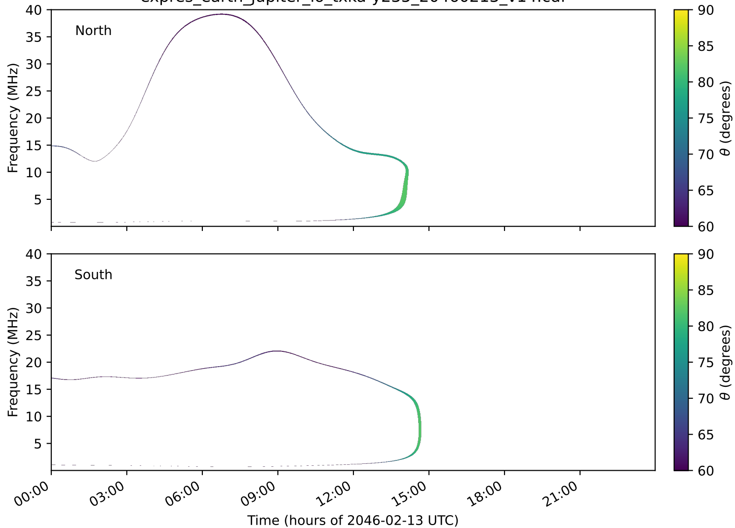
expres_earth_jupiter_io_txka-y235_20460213_v14.cdf
