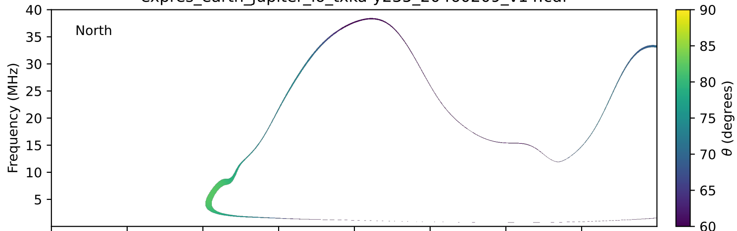
expres_earth_jupiter_io_txka-y235_20460209_v14.cdf
