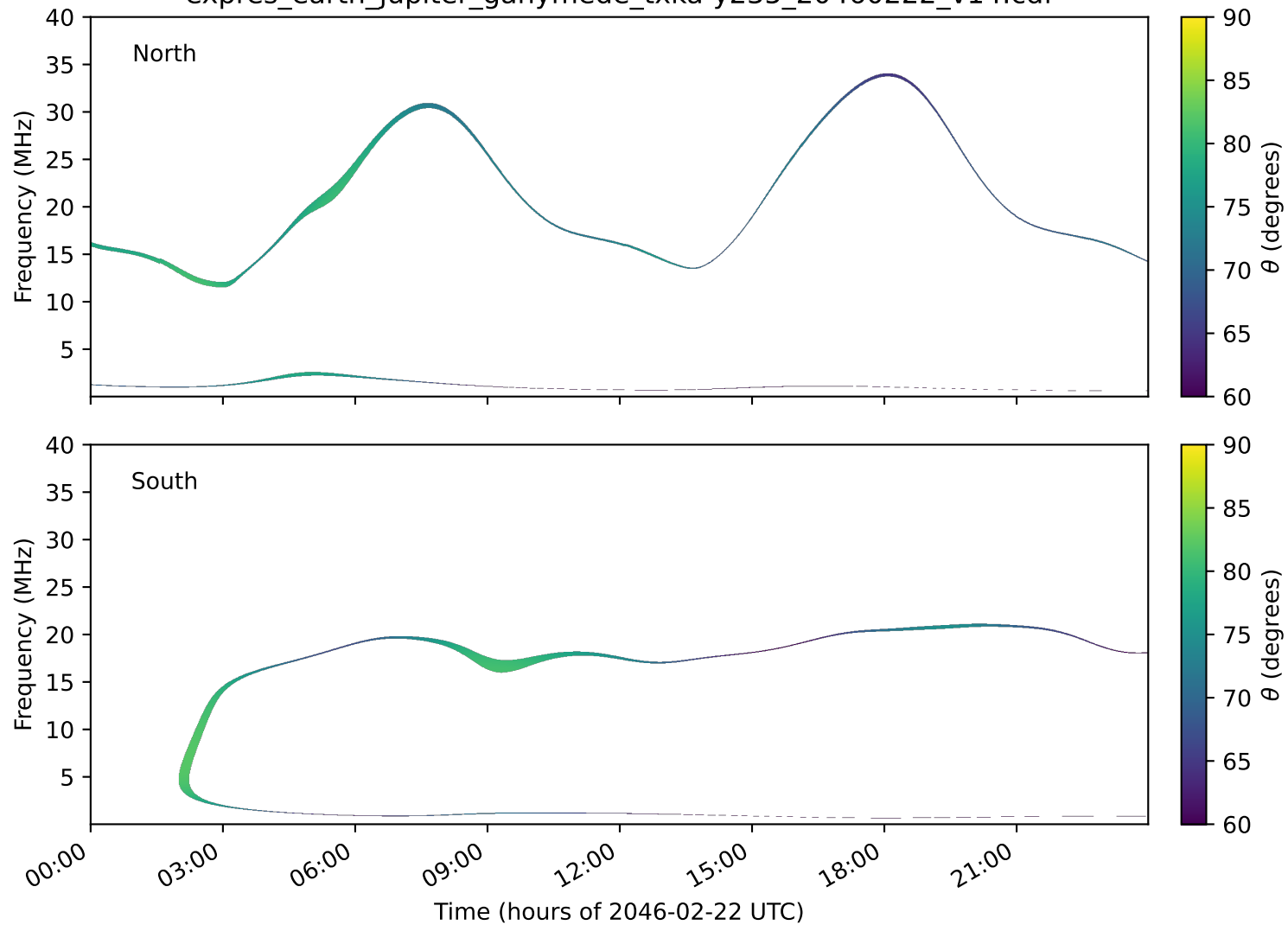
expres_earth_jupiter_ganymede_txka-y235_20460222_v14.cdf
