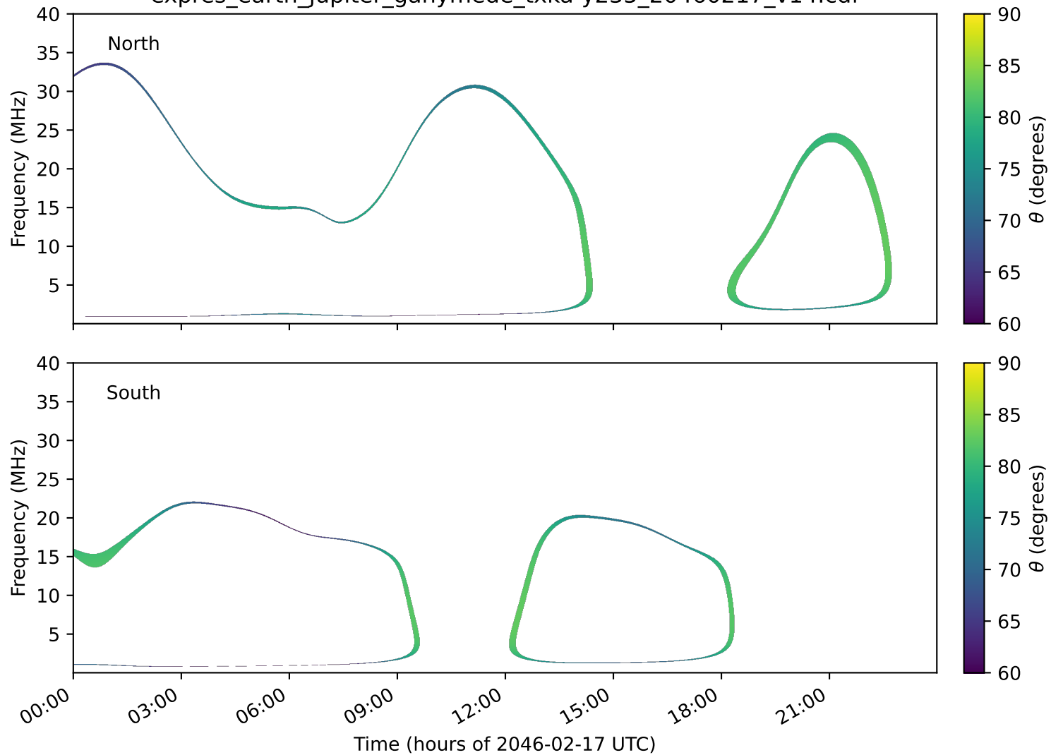
expres_earth_jupiter_ganymede_txka-y235_20460217_v14.cdf
