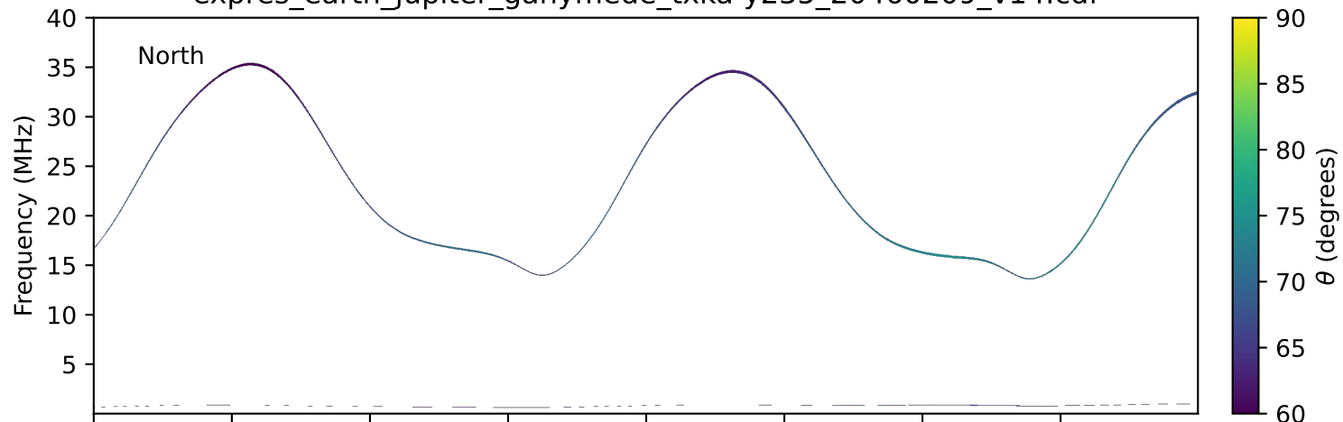
expres_earth_jupiter_ganymede_txka-y235_20460209_v14.cdf
