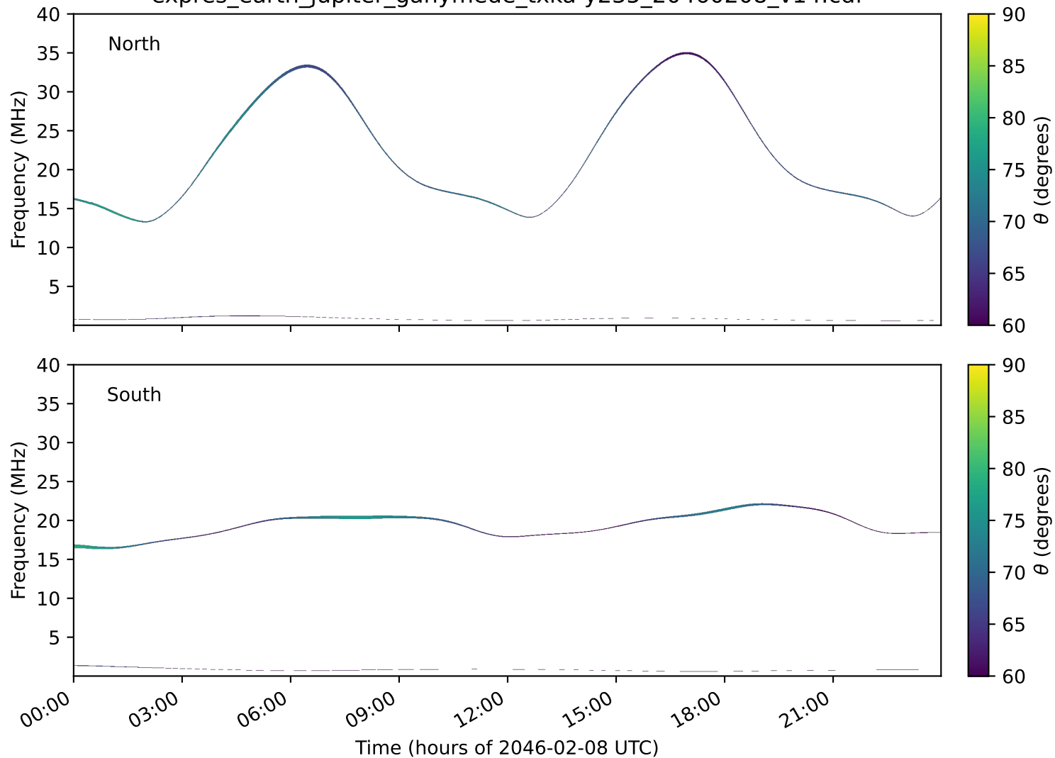
expres_earth_jupiter_ganymede_txka-y235_20460208_v14.cdf
