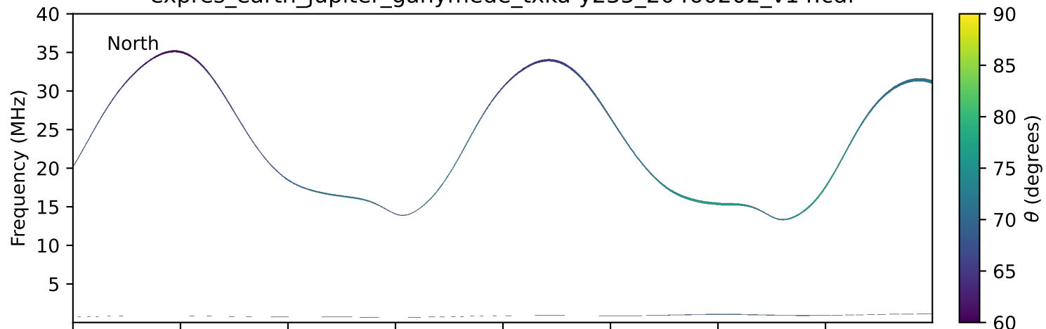
expres_earth_jupiter_ganymede_txka-y235_20460202_v14.cdf
