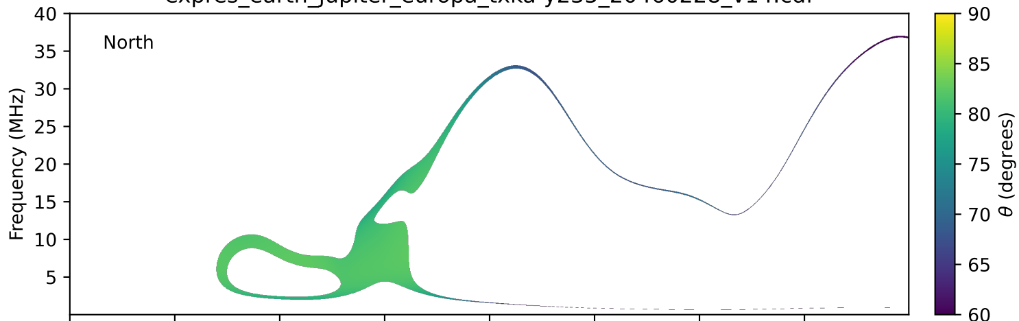
expres_earth_jupiter_europa_txka-y235_20460228_v14.cdf
