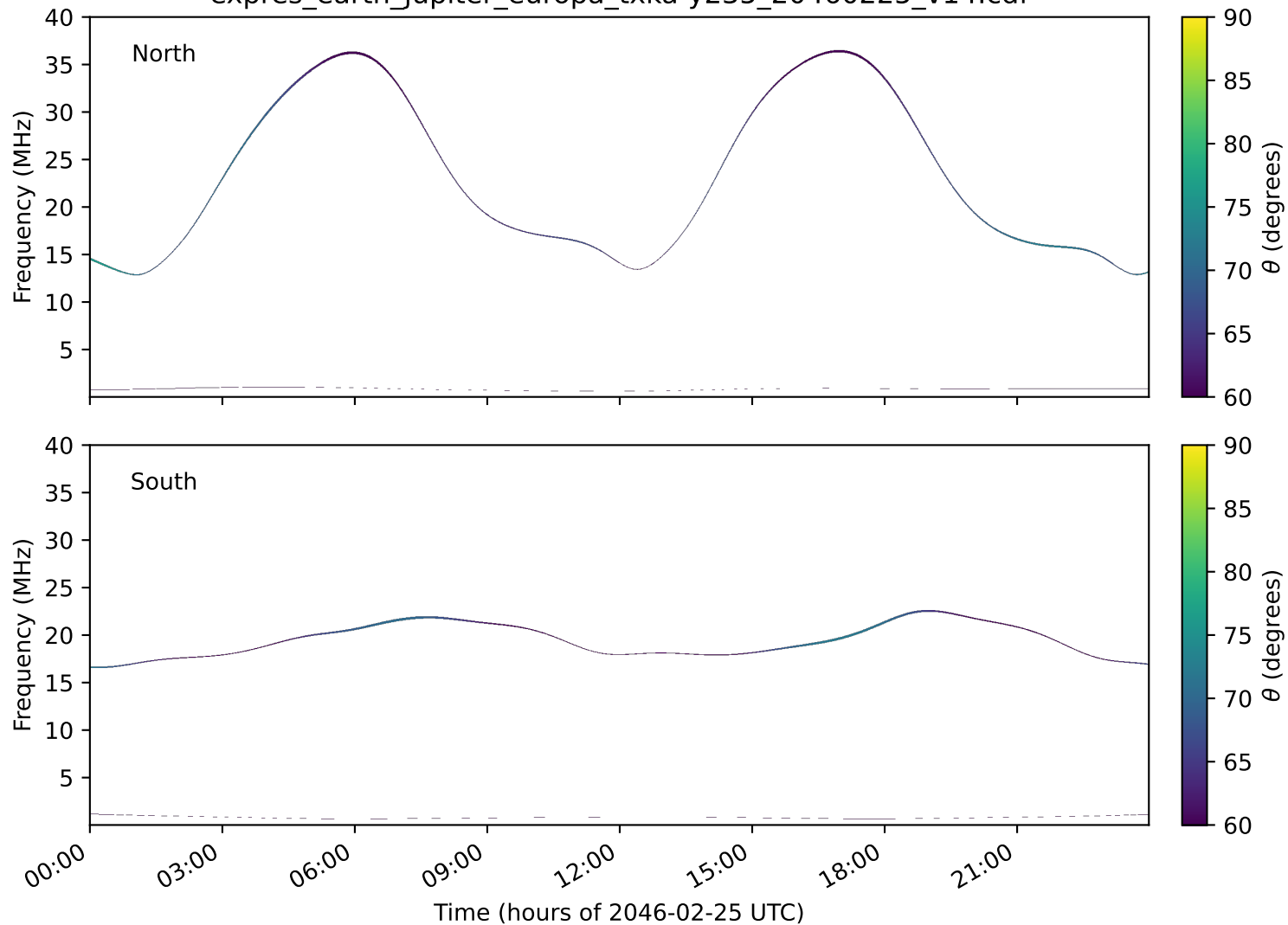
expres_earth_jupiter_europa_txka-y235_20460225_v14.cdf
