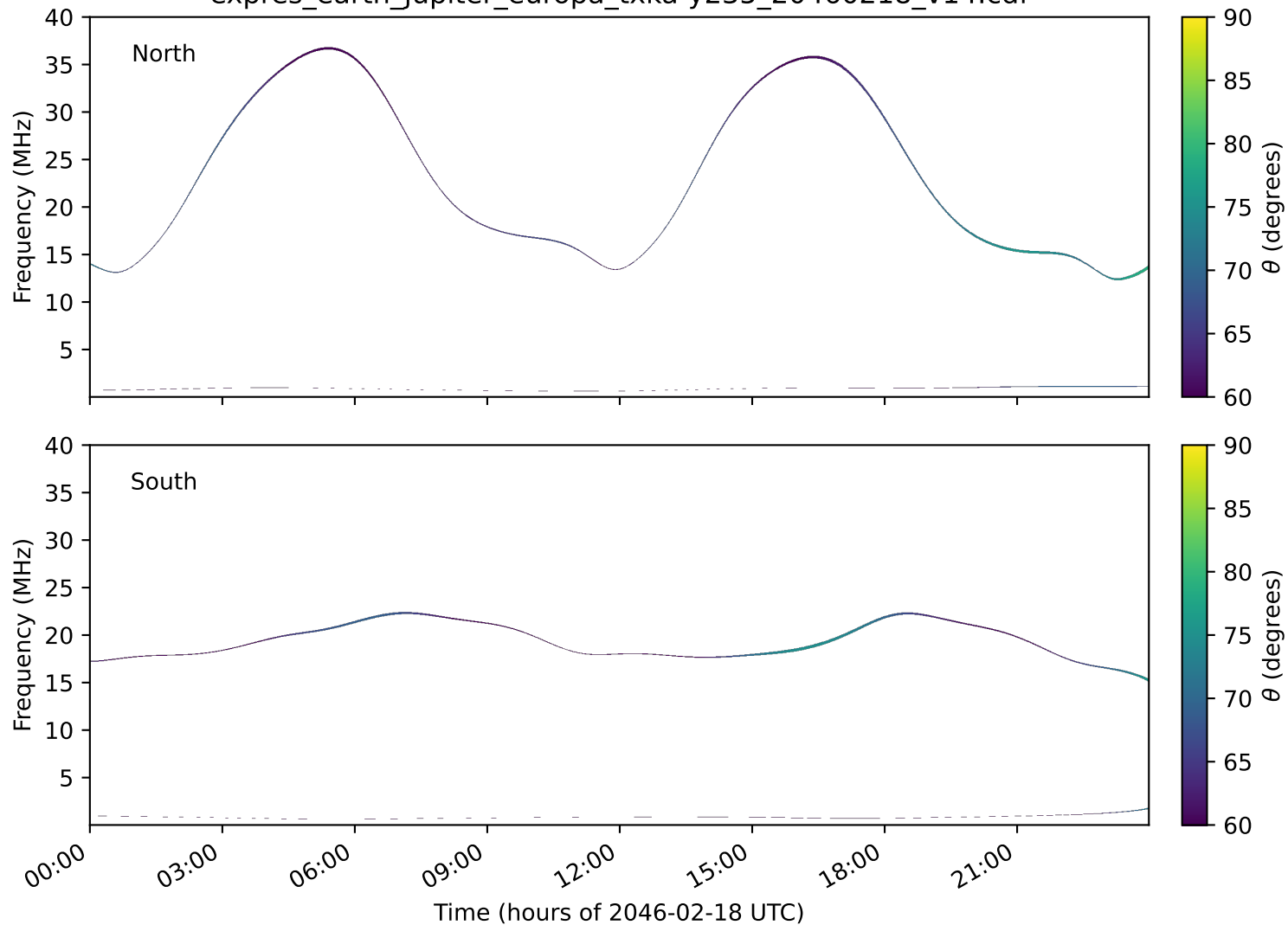
expres_earth_jupiter_europa_txka-y235_20460218_v14.cdf
