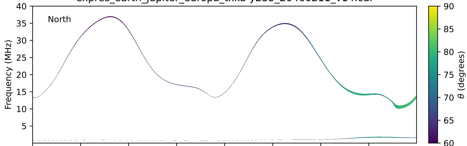
expres_earth_jupiter_europa_txka-y235_20460211_v14.cdf
