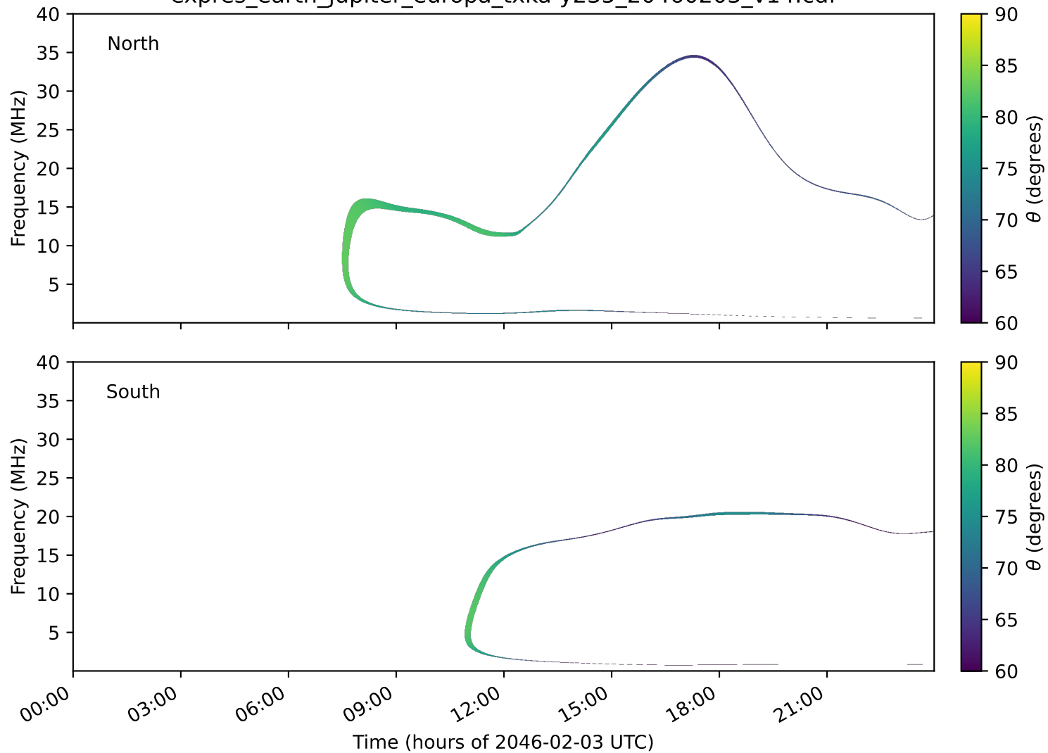
expres_earth_jupiter_europa_txka-y235_20460203_v14.cdf
